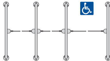
Double lane SLIMLANE 940 + Single lane SLIMLANE 950
