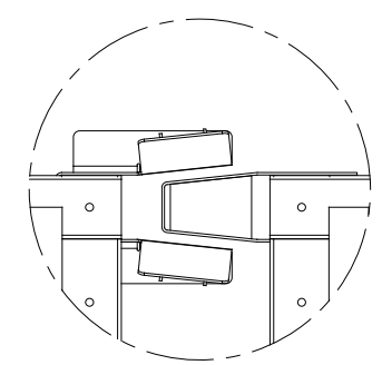
DETAIL "A" INTERLOCK OPTION FOR MASTER/SLAVE
